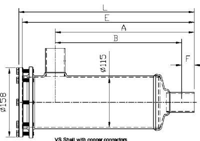
VS Shell with copper connectors
